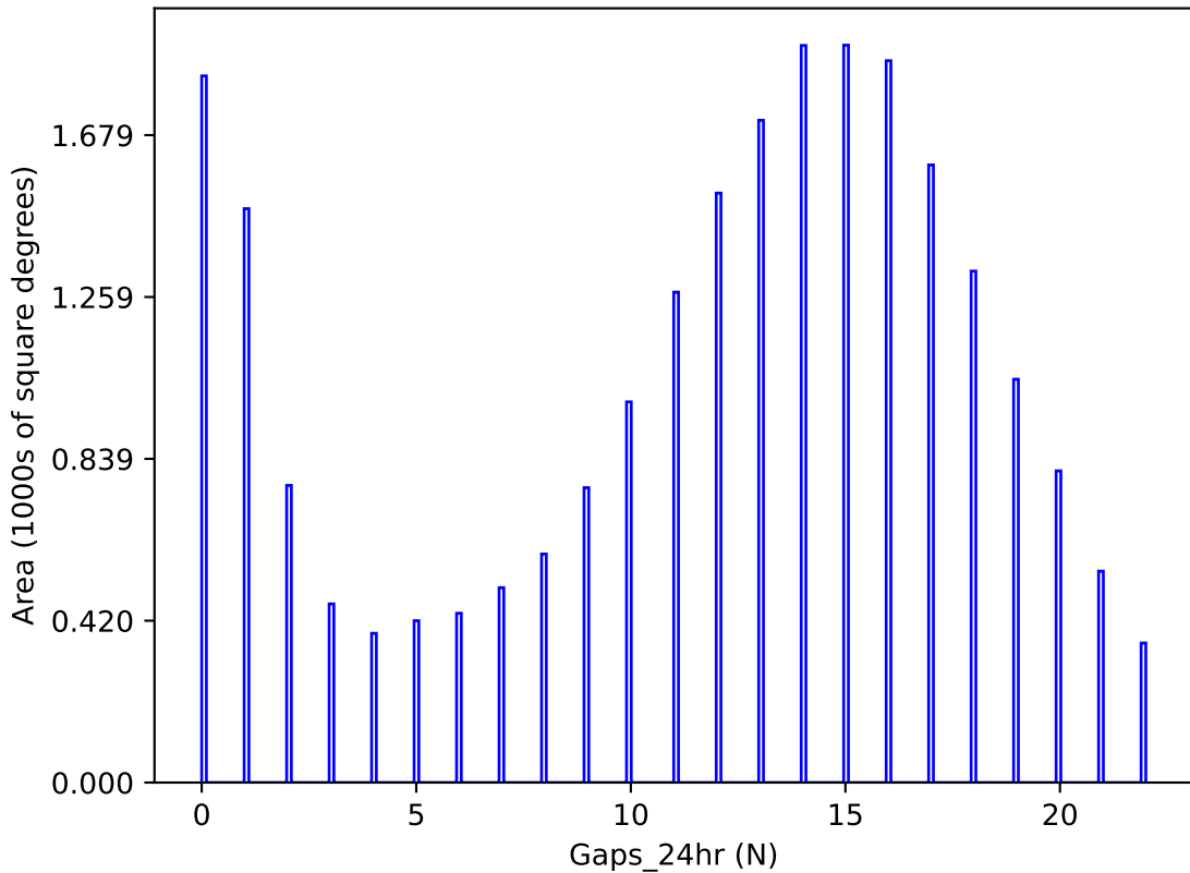
weather_cloudso1v3.4_10yrs y band: Gaps_24hr
