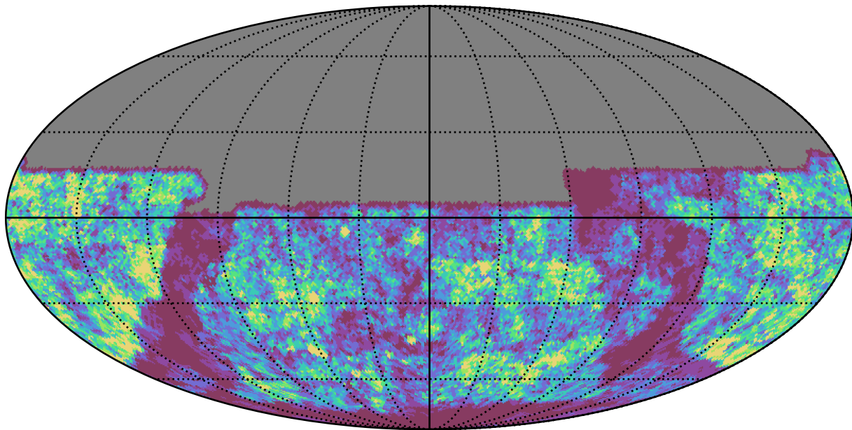
weather_cloudso1v3.4_10yrs u band: Gaps_24hr
