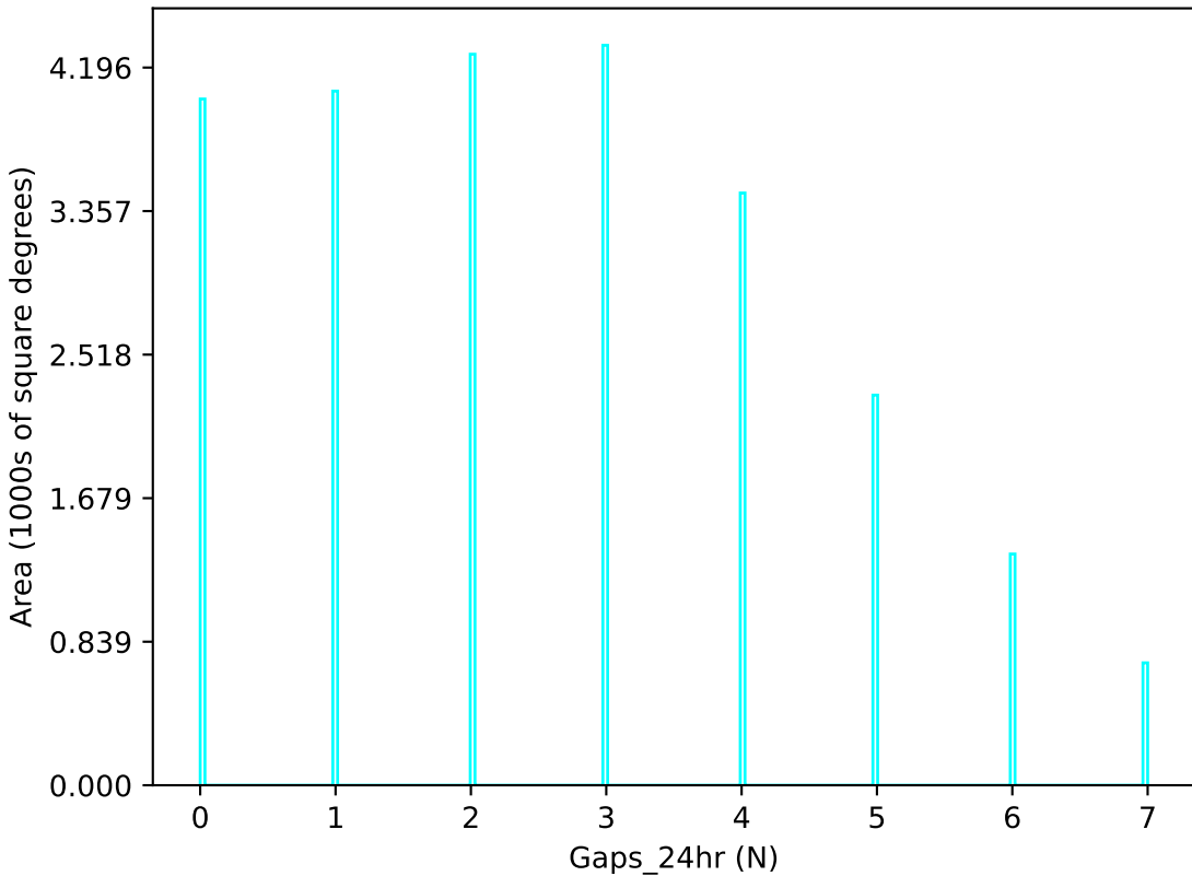
weather_cloudso1v3.4_10yrs u band: Gaps_24hr
