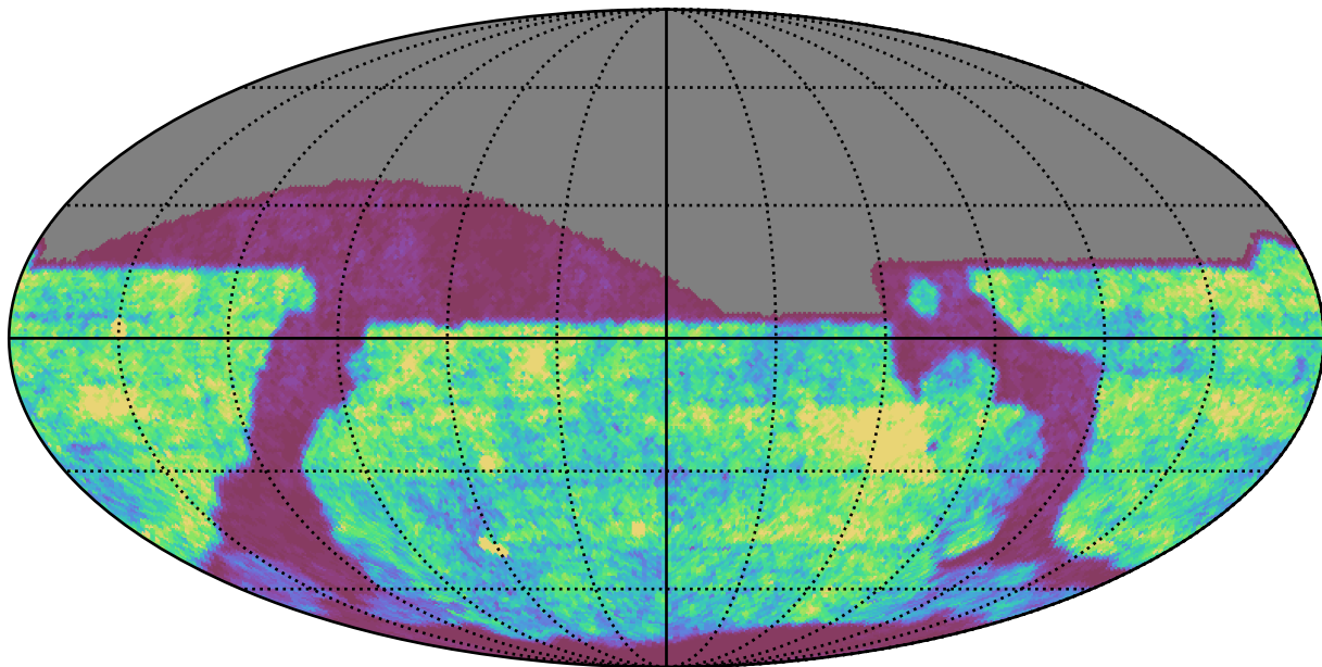
weather_cloudso1v3.4_10yrs r band: Gaps_24hr
