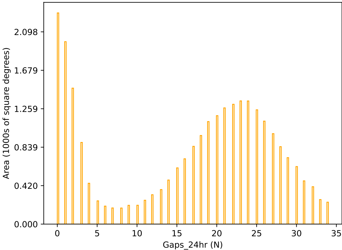
weather_cloudso1v3.4_10yrs r band: Gaps_24hr
