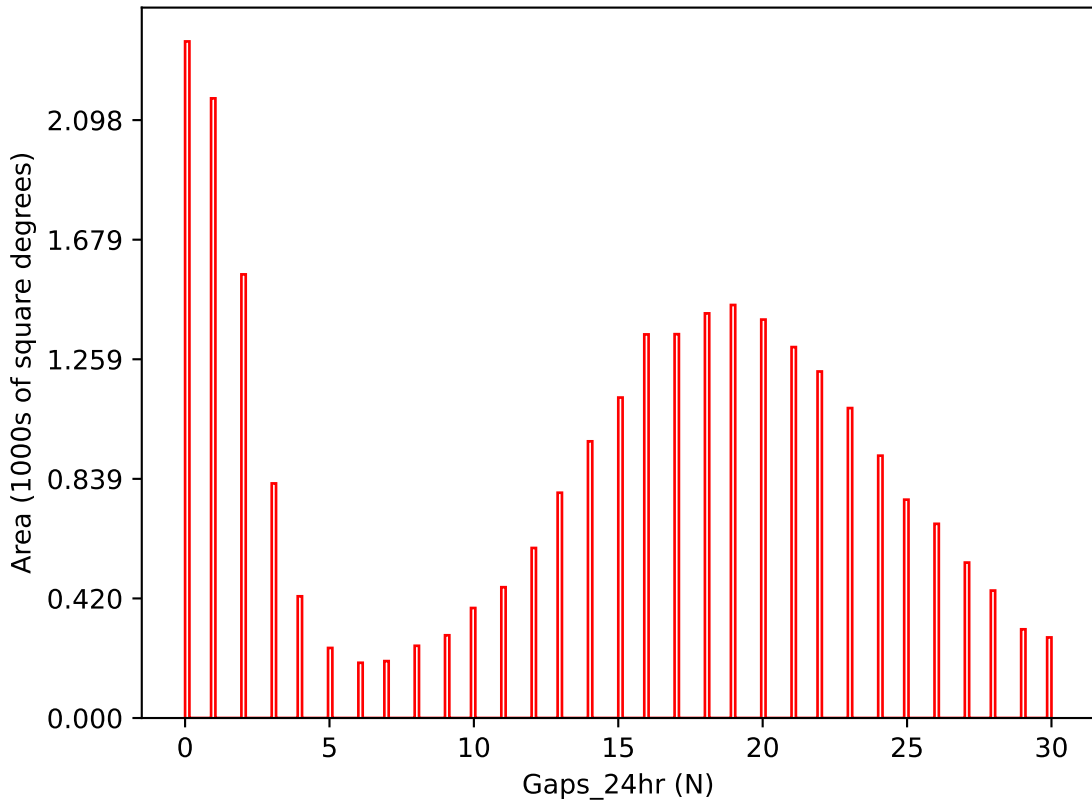
weather_cloudso1v3.4_10yrs i band: Gaps_24hr
