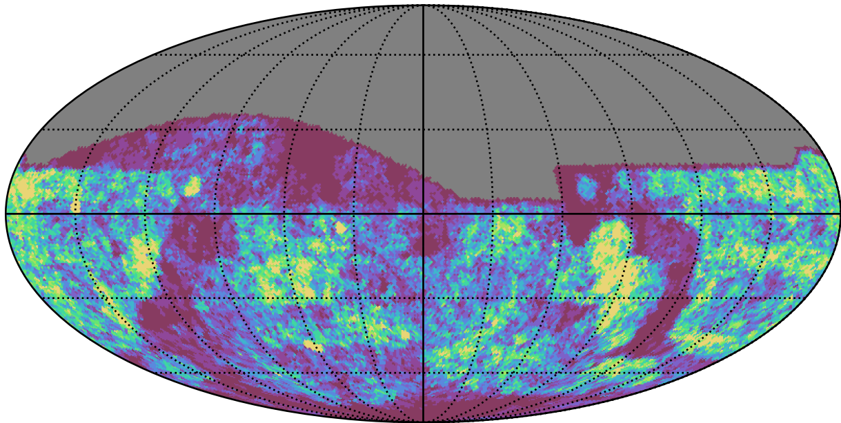
weather_cloudso1v3.4_10yrs g band: Gaps_24hr
