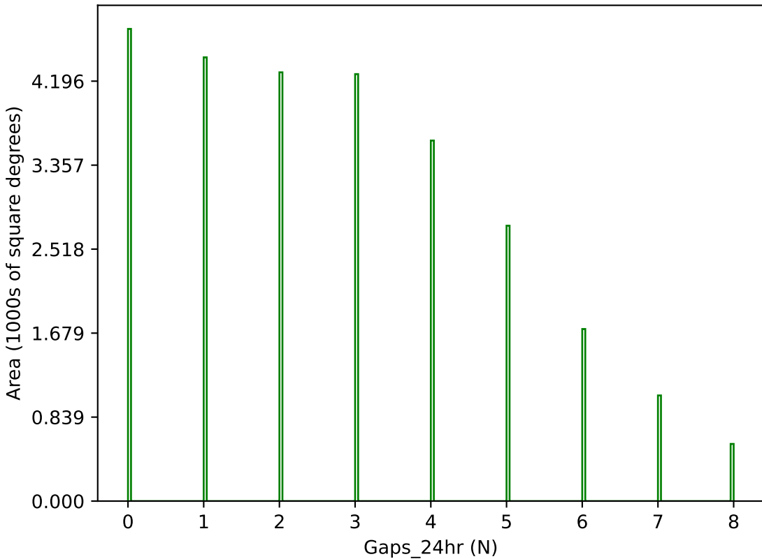
weather_cloudso1v3.4_10yrs g band: Gaps_24hr
