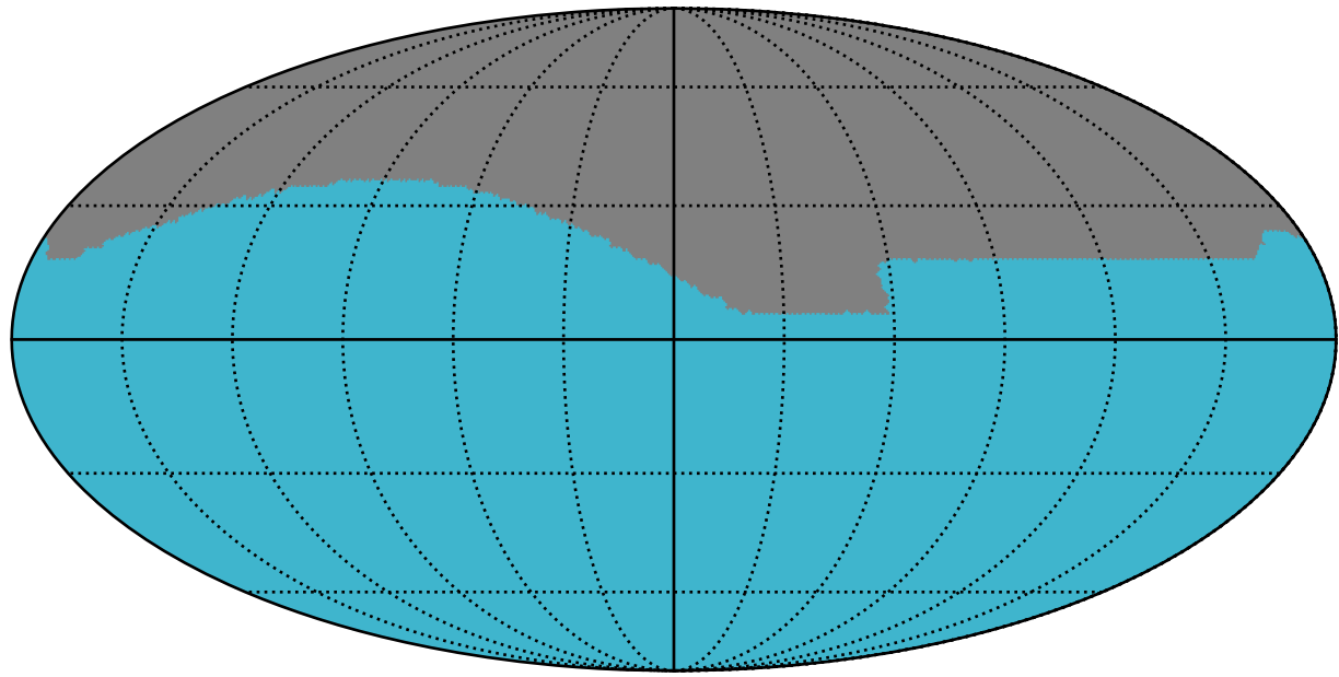
weather_cloudso1v3.4_10yrs : GalplaneFootprintMetric_xray_binaries_map_Tau_2_0
