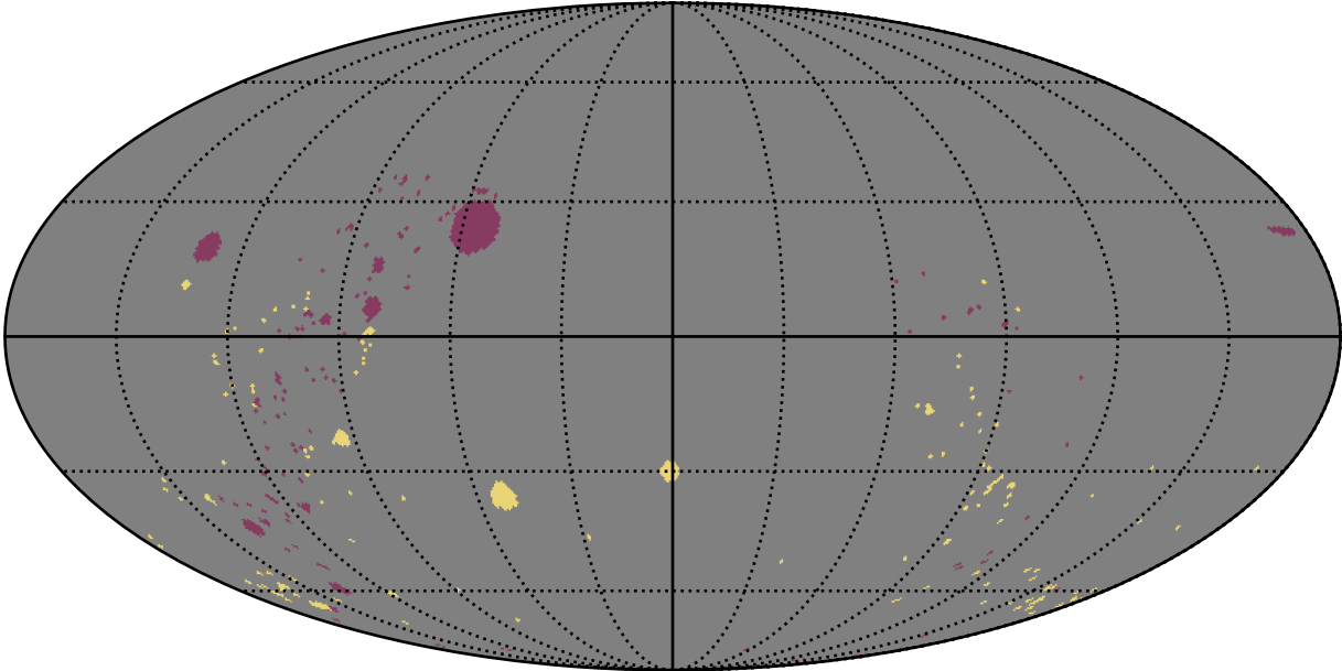
weather_cloudso1v3.4_10yrs : GalplaneFootprintMetric_open_clusters_map_Tau_11_0
