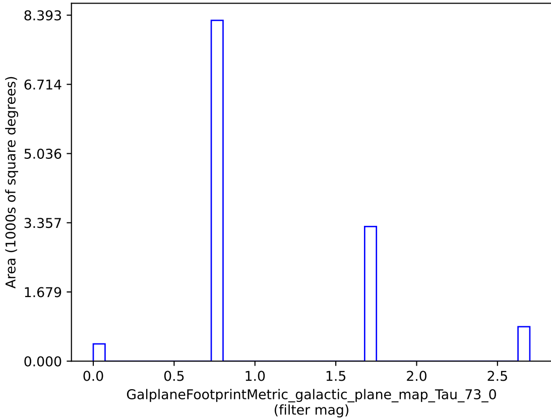
weather_cloudso1v3.4_10yrs : GalplaneFootprintMetric_galactic_plane_map_Tau_73_0
