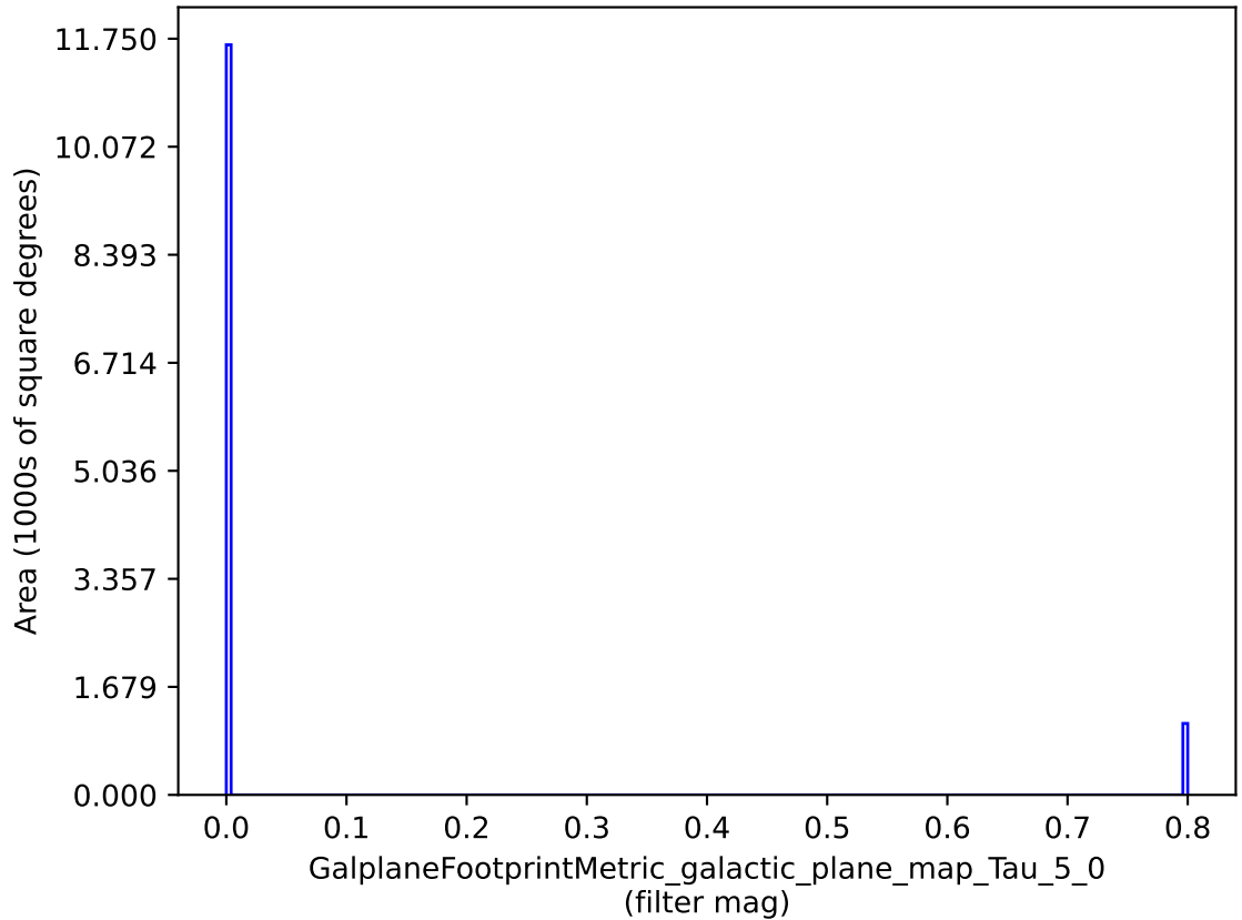
weather_cloudso1v3.4_10yrs : GalplaneFootprintMetric_galactic_plane_map_Tau_5_0
