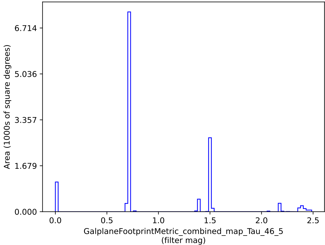
weather_cloudso1v3.4_10yrs : GalplaneFootprintMetric_combined_map_Tau_46_5
