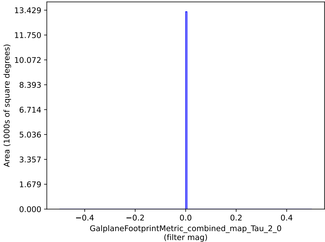
weather_cloudso1v3.4_10yrs : GalplaneFootprintMetric_combined_map_Tau_2_0
