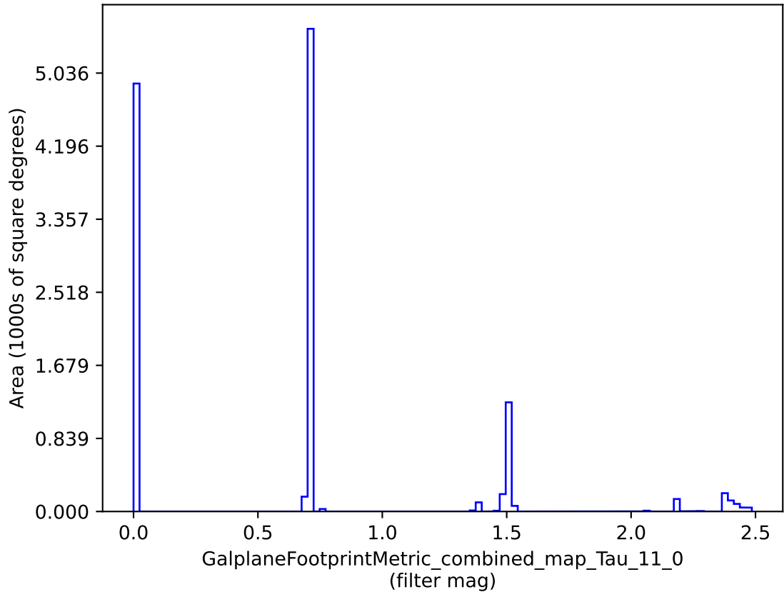
weather_cloudso1v3.4_10yrs : GalplaneFootprintMetric_combined_map_Tau_11_0
