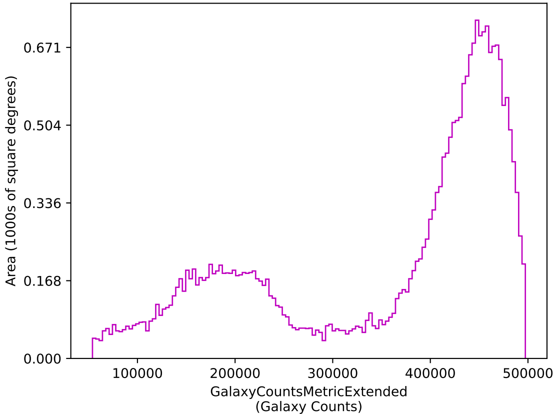
weather_cloudso1v3.4_10yrs z: GalaxyCountsMetricExtended
