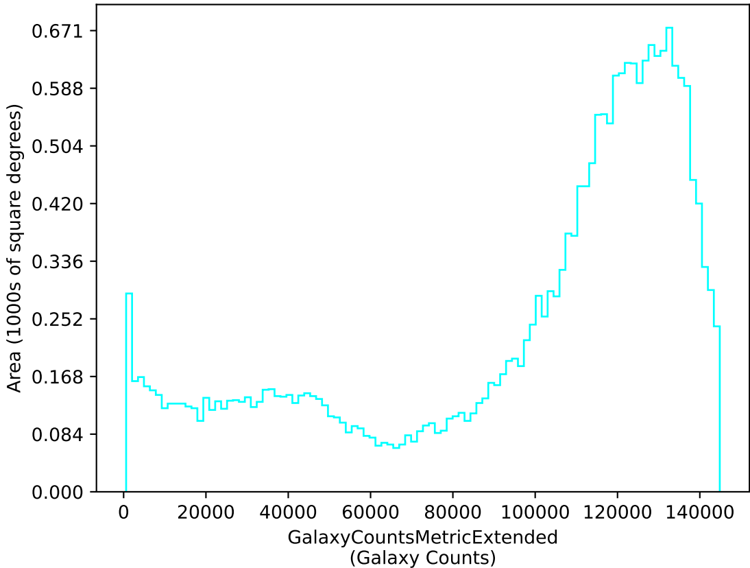
weather_cloudso1v3.4_10yrs u: GalaxyCountsMetricExtended
