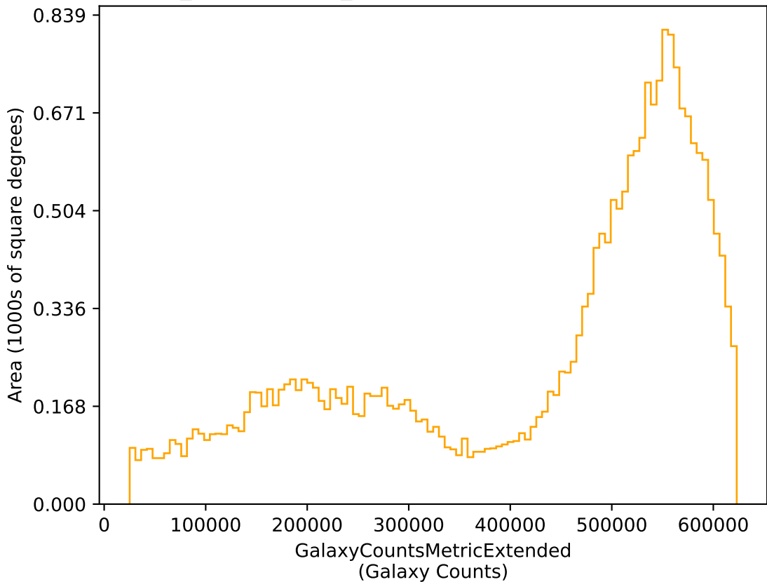
weather_cloudso1v3.4_10yrs r: GalaxyCountsMetricExtended
