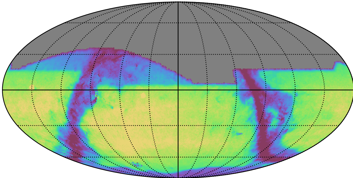
weather_cloudso1v3.4_10yrs i: GalaxyCountsMetricExtended
