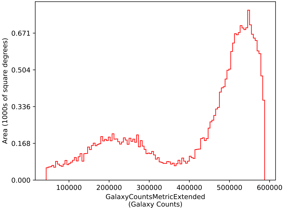
weather_cloudso1v3.4_10yrs i: GalaxyCountsMetricExtended
