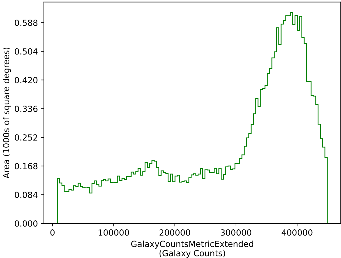
weather_cloudso1v3.4_10yrs g: GalaxyCountsMetricExtended
