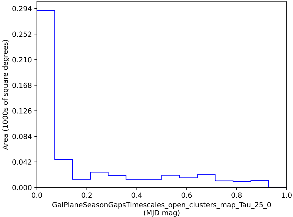
weather_cloudso1v3.4_10yrs : GalPlaneSeasonGapsTimescales_open_clusters_map_Tau_25_0
