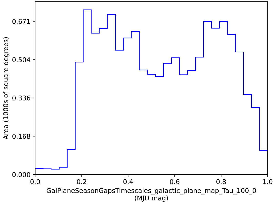
weather_cloudso1v3.4_10yrs : GalPlaneSeasonGapsTimescales_galactic_plane_map_Tau_100_0
