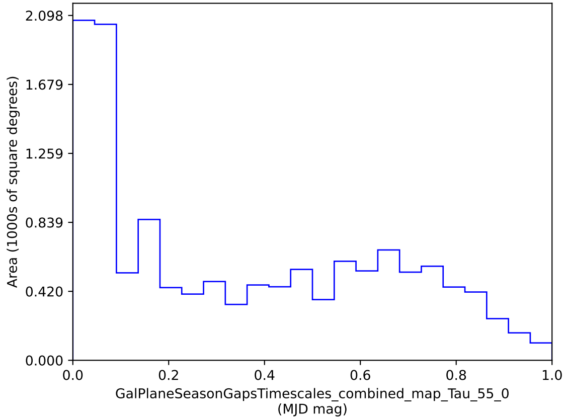
weather_cloudso1v3.4_10yrs : GalPlaneSeasonGapsTimescales_combined_map_Tau_55_0
