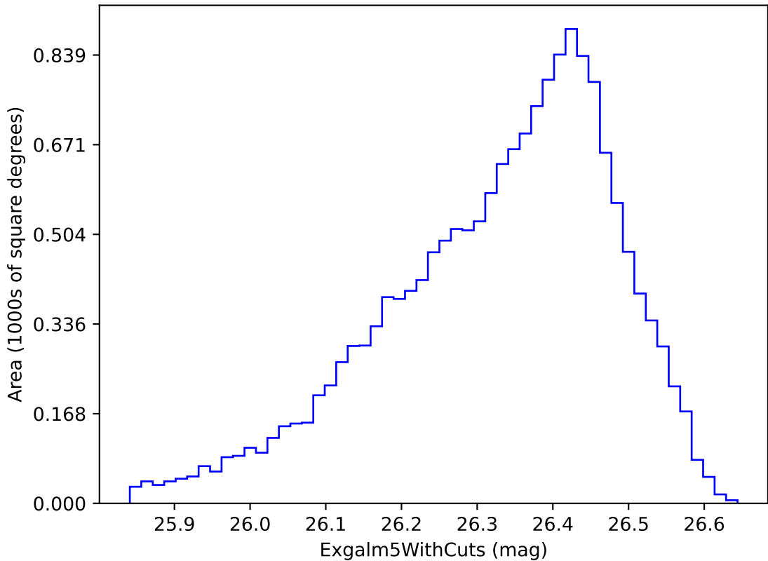
weather_cloudso1v3.4_10yrs i band non-DD year 9: Exgalml5WithCuts
