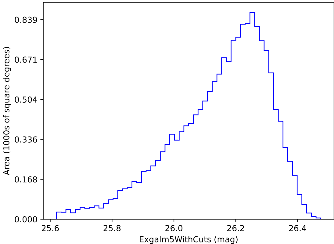
weather_cloudso1v3.4_10yrs i band non-DD year 6: Exgal5WithCuts
