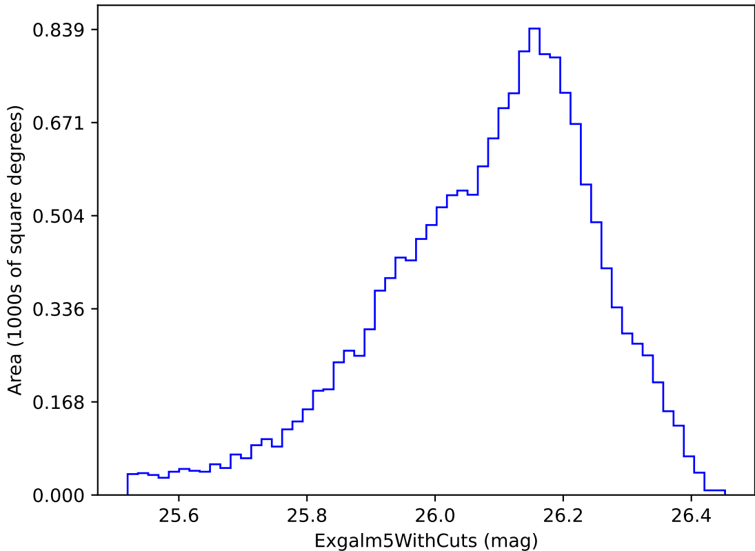
weather_cloudso1v3.4_10yrs i band non-DD year 5: Exgalml5WithCuts
