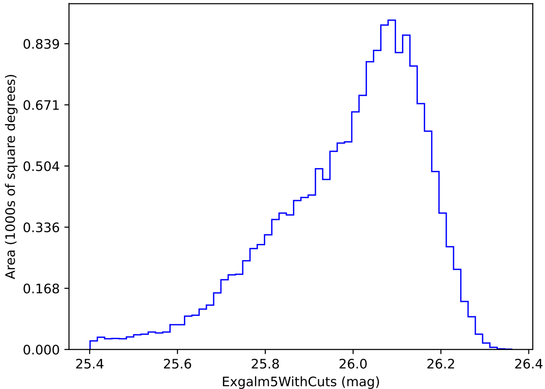
weather_cloudso1v3.4_10yrs i band non-DD year 4: Exgalml5WithCuts
