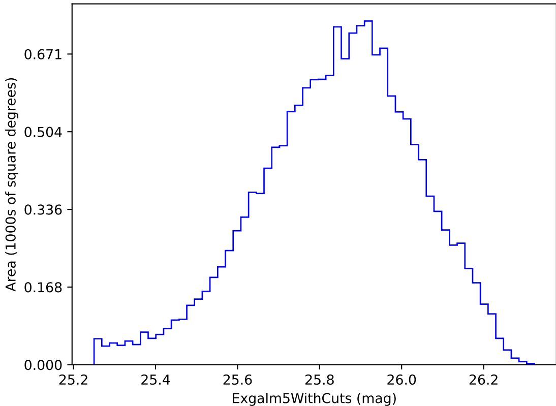
weather_cloudso1v3.4_10yrs i band non-DD year 3: ExgalM5WithCuts
