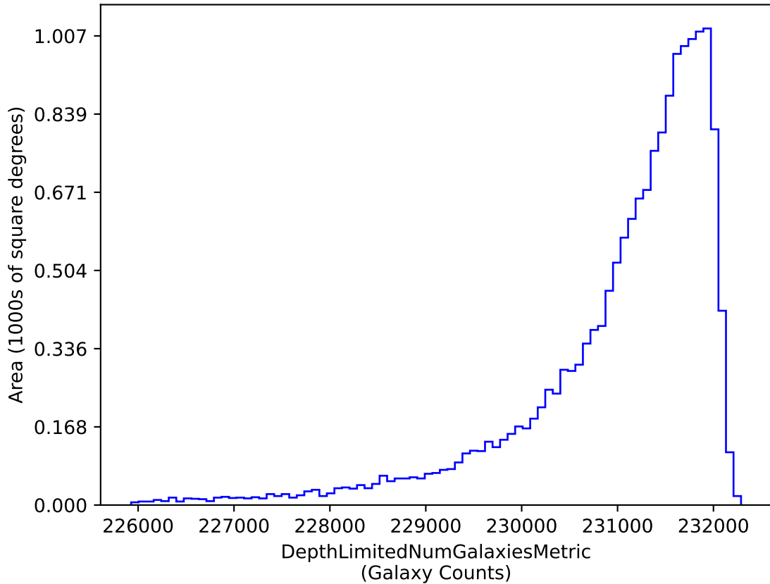
weather_cloudso1v3.4_10yrs i band galaxies non-DD: DepthLimitedNumGalaxiesMetric
