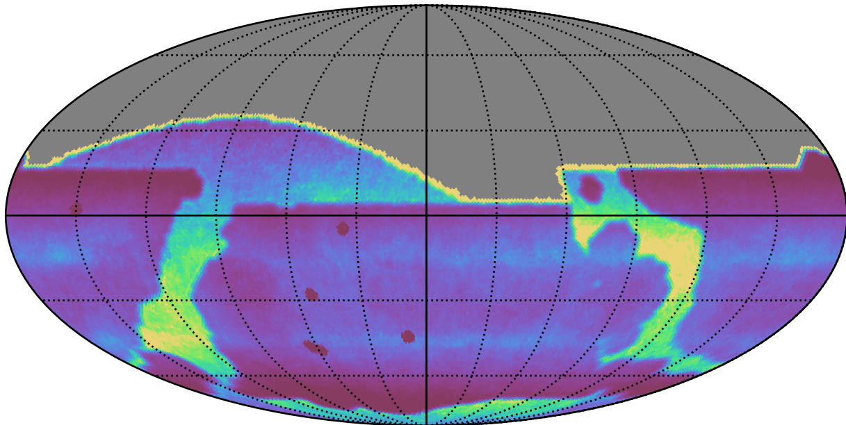
weather_cloudso1v3.4_10yrs : DCRprecision
