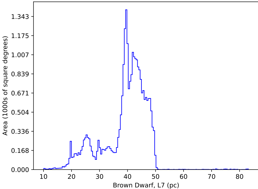
weather_cloudso1v3.4_10yrs : Brown Dwarf, L7
