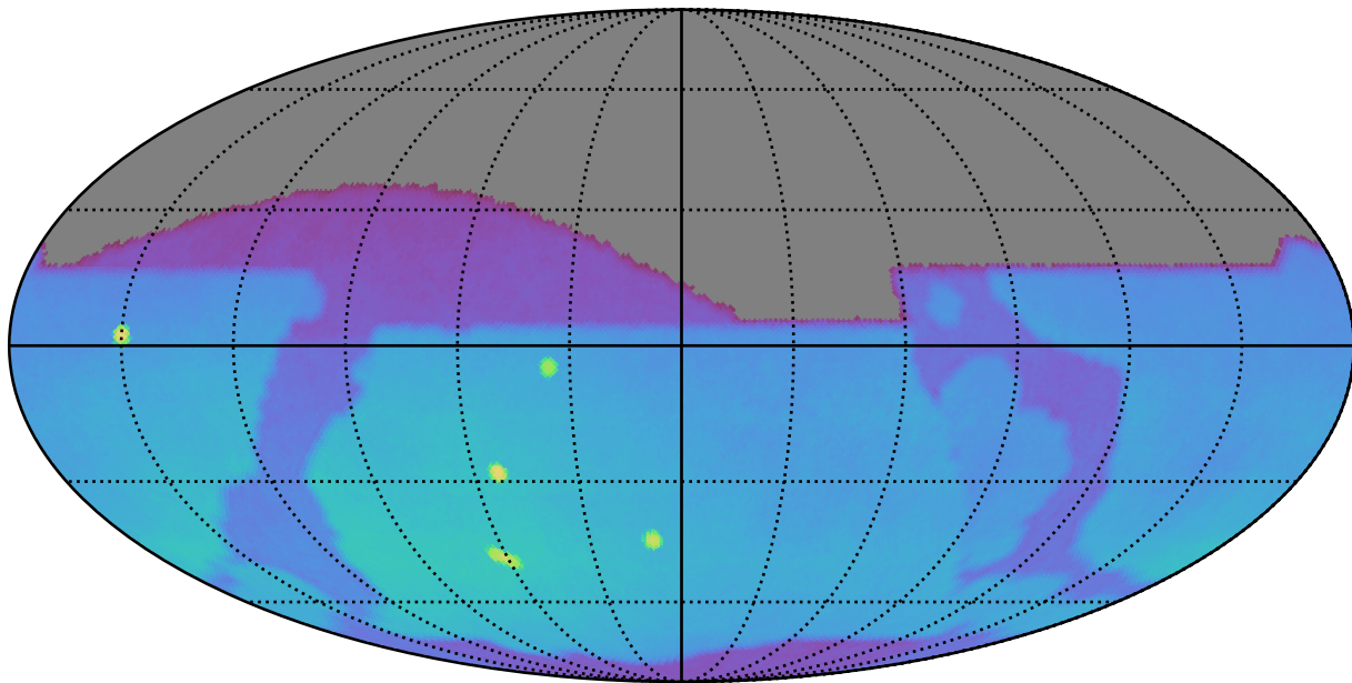
weather_cloudso1v3.4_10yrs : Brown Dwarf, L4
