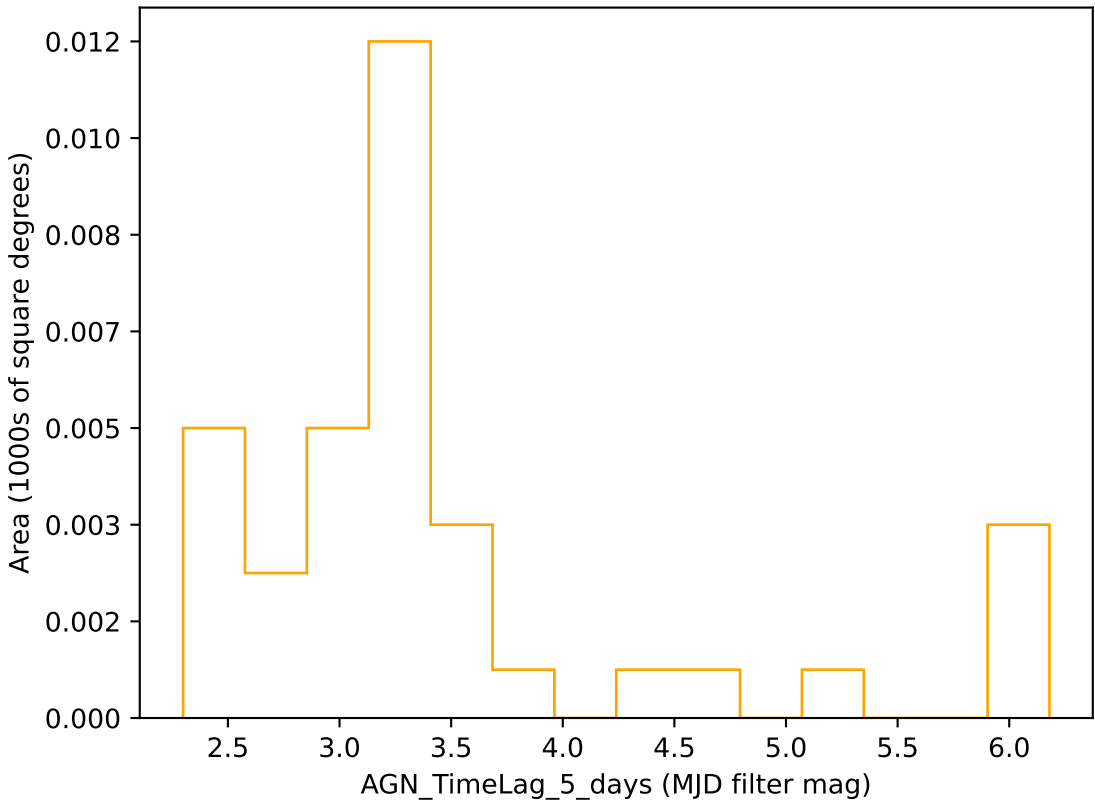
weather_cloudso1v3.4_10yrs r band: AGN_TimeLag_5_days
