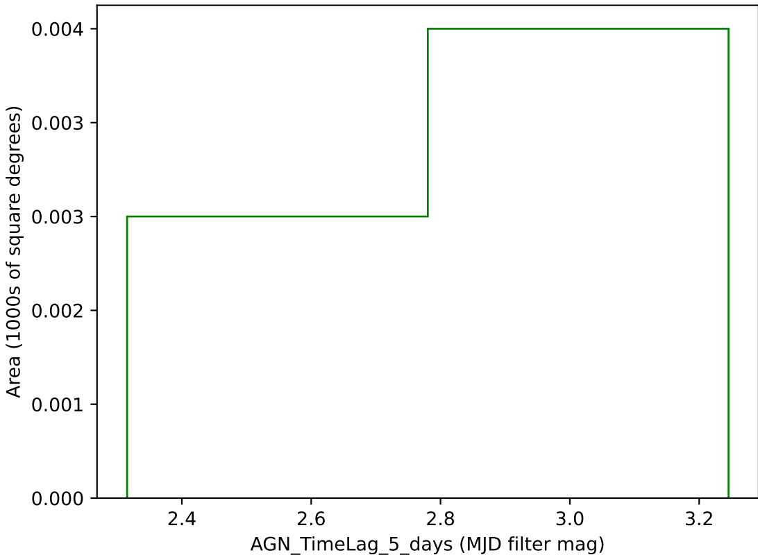
weather_cloudso1v3.4_10yrs g band: AGN_TimeLag_5_days
