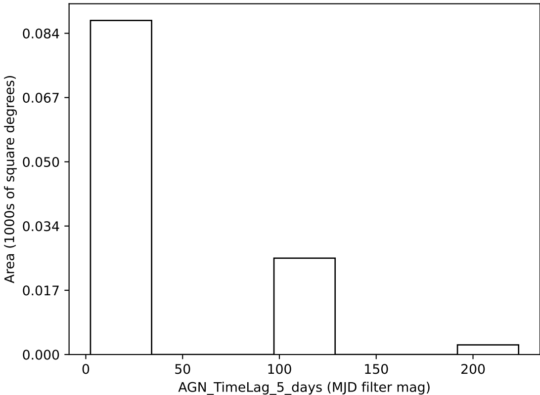
weather_cloudso1v3.4_10yrs all bands: AGN_TimeLag_5_days
