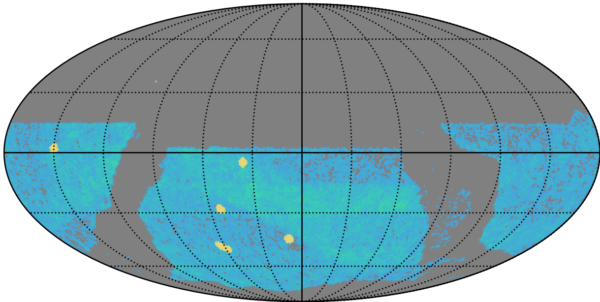
weather_cloudso1v3.4_10yrs z band: AGN_TimeLag_100_days
