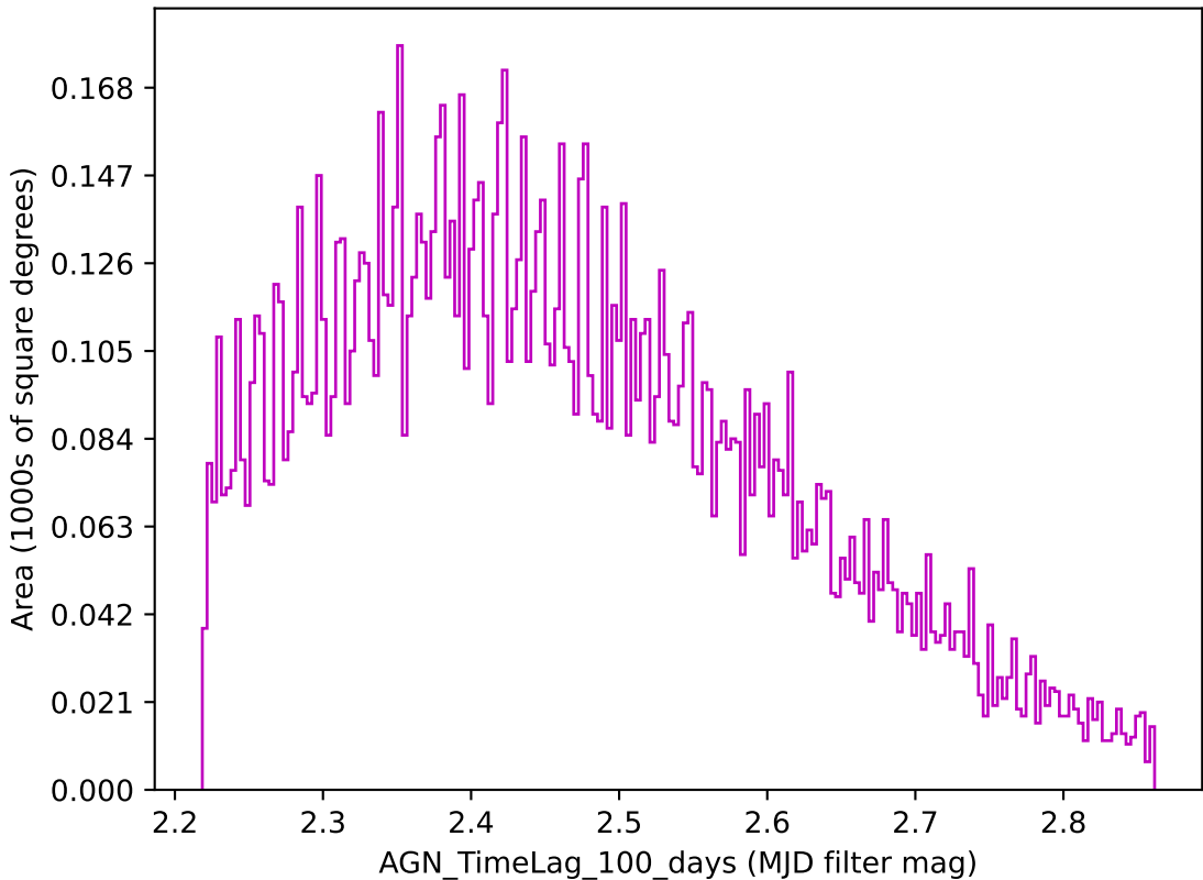
weather_cloudso1v3.4_10yrs z band: AGN_TimeLag_100_days
