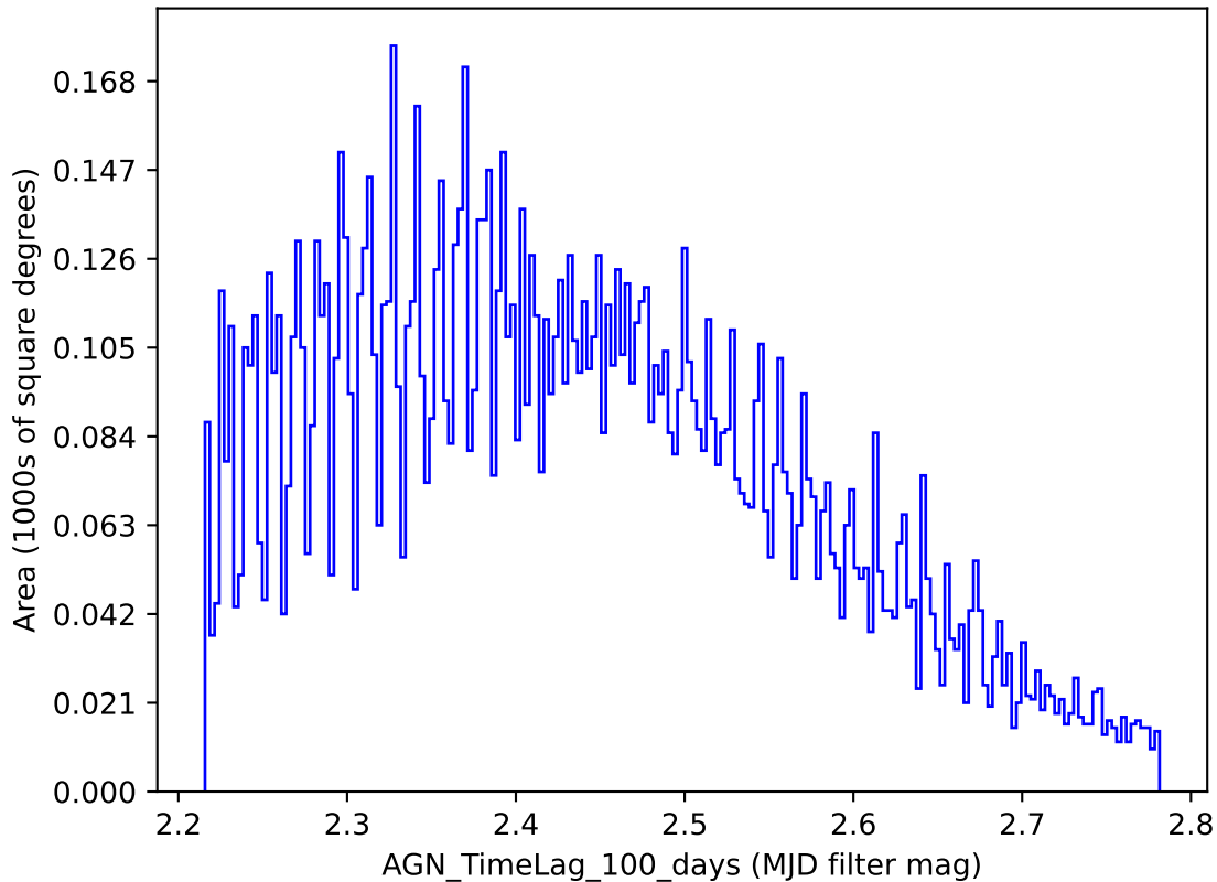
weather_cloudso1v3.4_10yrs y band: AGN_TimeLag_100_days
