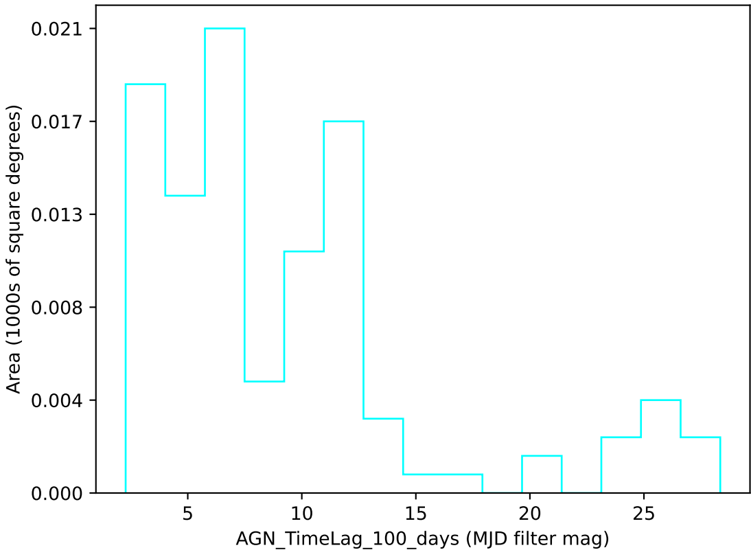
weather_cloudso1v3.4_10yrs u band: AGN_TimeLag_100_days
