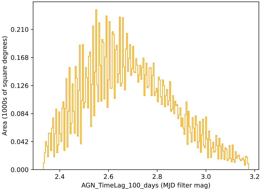
weather_cloudso1v3.4_10yrs r band: AGN_TimeLag_100_days
