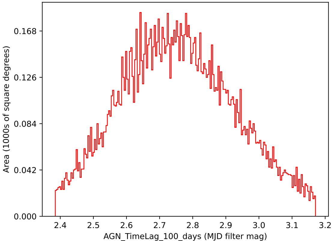
weather_cloudso1v3.4_10yrs i band: AGN_TimeLag_100_days
