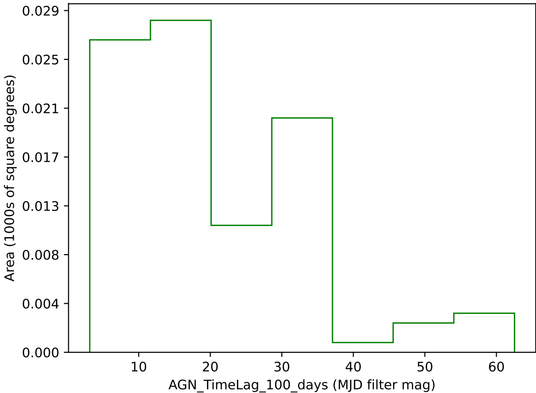
weather_cloudso1v3.4_10yrs g band: AGN_TimeLag_100_days
