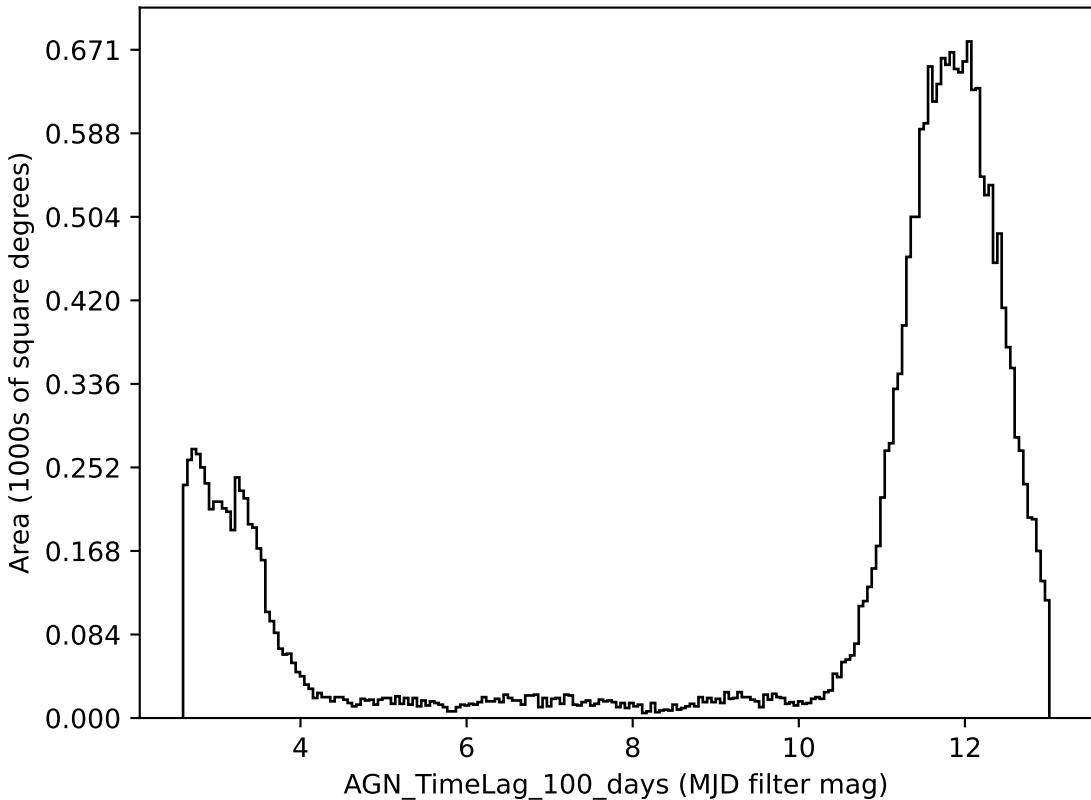
weather_cloudso1v3.4_10yrs all bands: AGN_TimeLag_100_days
