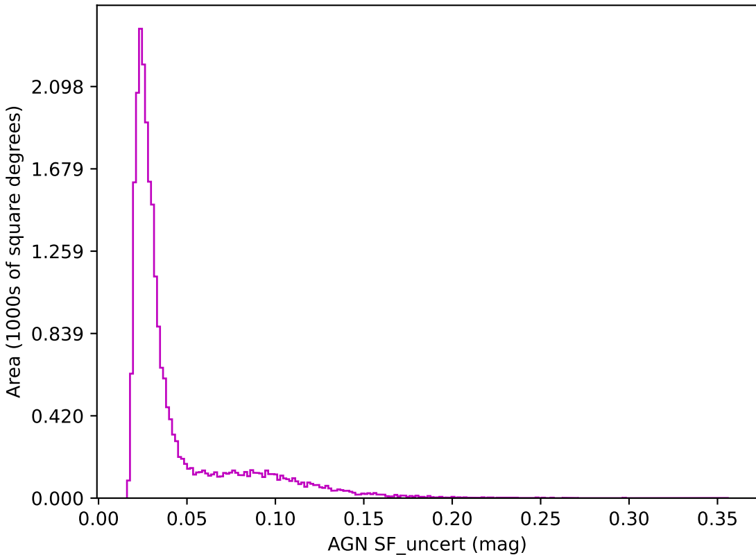
weather_cloudso1v3.4_10yrs z band: AGN SF_uncert
