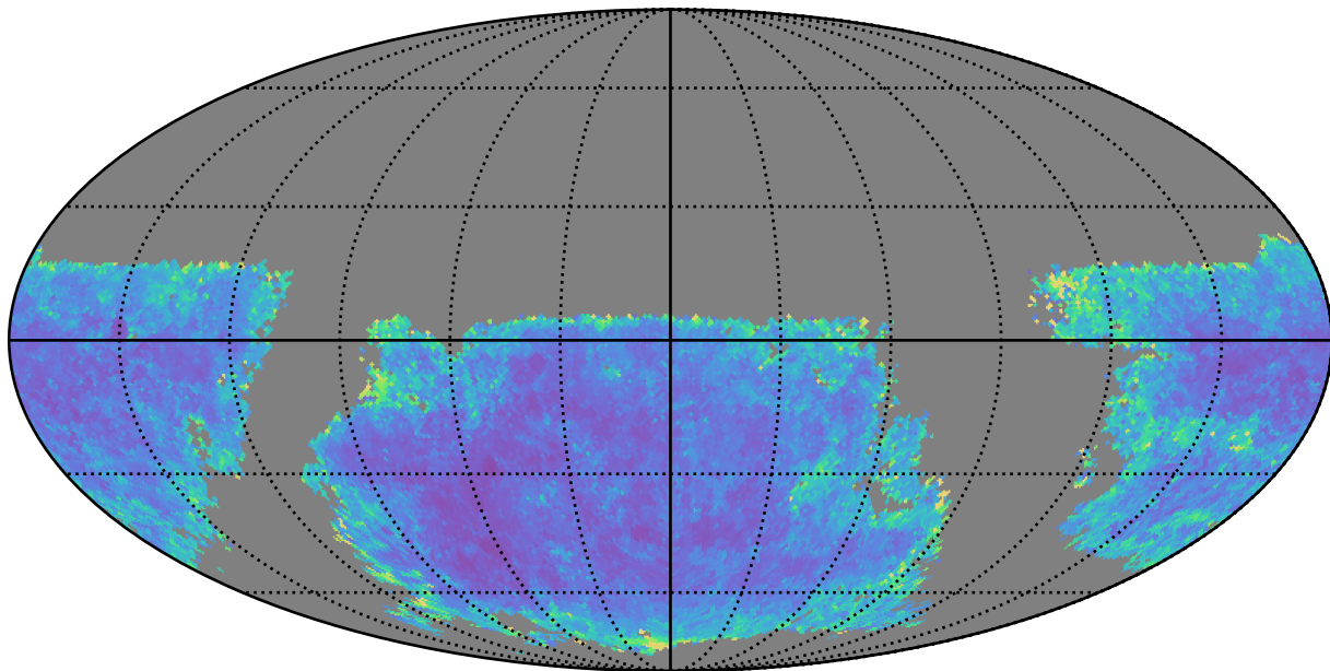
weather_cloudso1v3.4_10yrs u band: AGN SF_uncert
