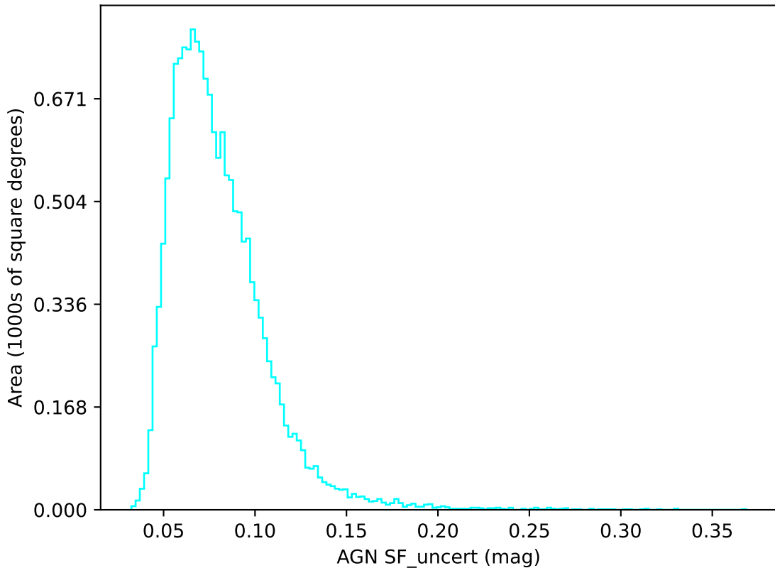
weather_cloudso1v3.4_10yrs u band: AGN SF_uncert
