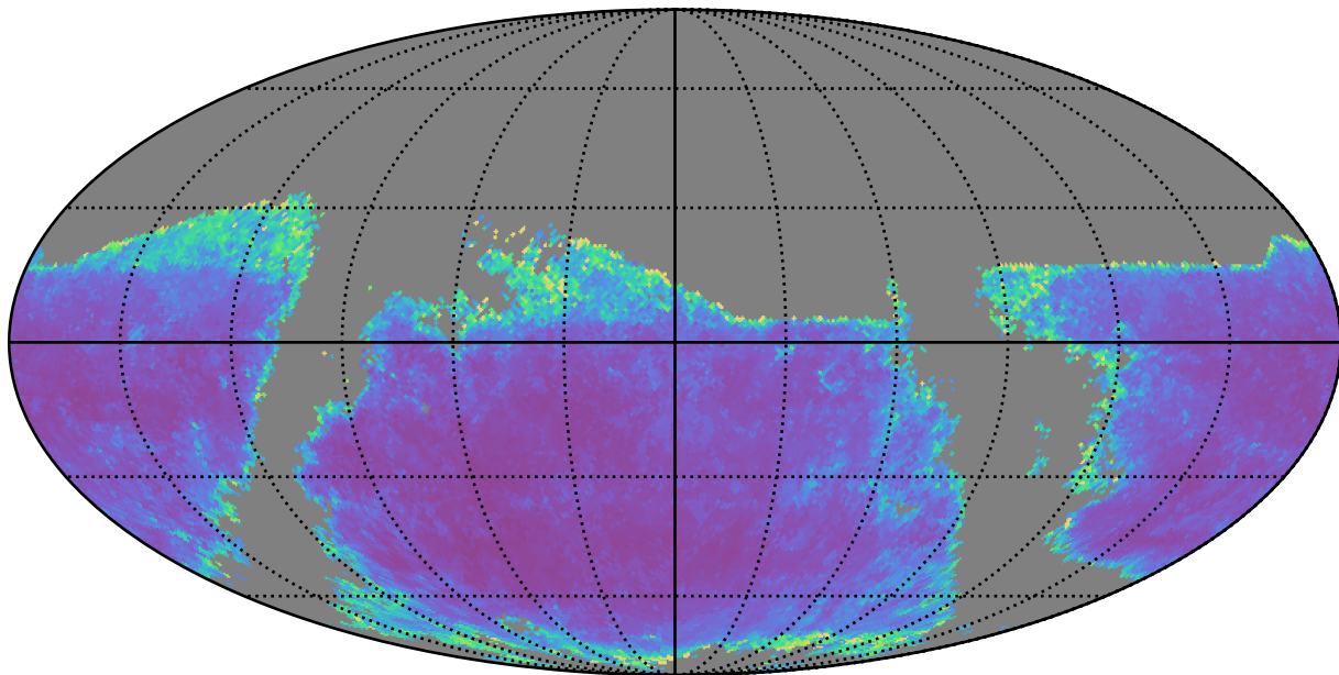
weather_cloudso1v3.4_10yrs g band: AGN SF_uncert
