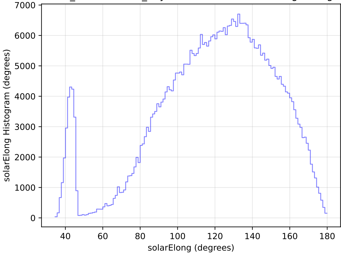
weather_cloudso1v3.4_10yrs WFD z band: solarElong Histogram
