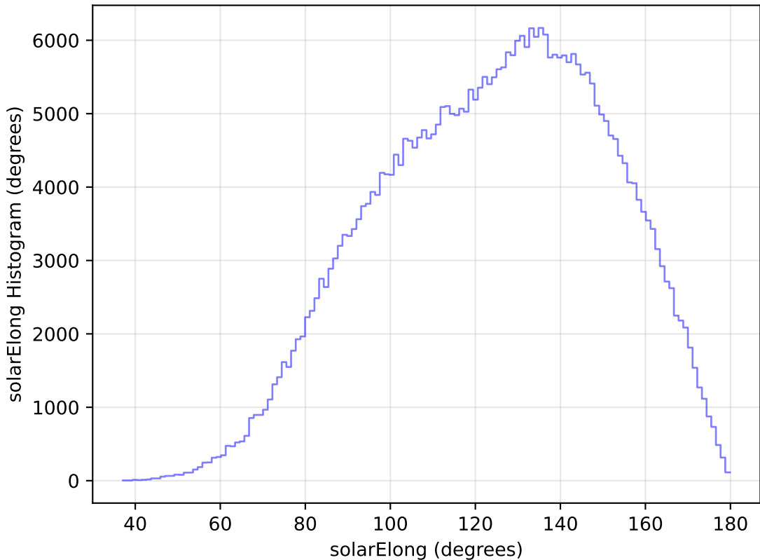
weather_cloudso1v3.4_10yrs WFD y band: solarElong Histogram
